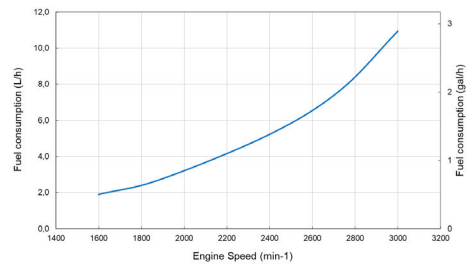
4JH5E Fuel consumption (propload exp 3.0)
